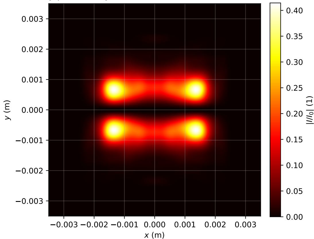
Intensity profile I(x, y, z = 3.025)/I_0 , P_{in}=4.0P_{cr} , artificial time
